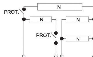
41XX70 -22 ( 7000 W )
