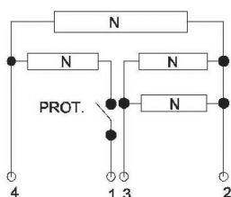
41XX50 -21 (5000 W)
